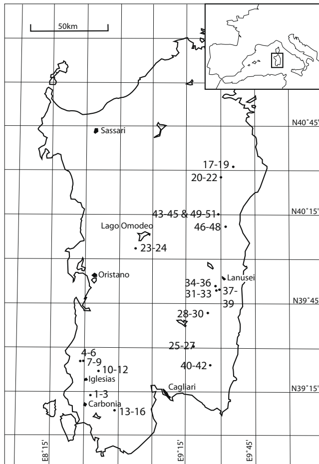
Fig. 1. Sampling localities for all Sardinian species. Numbers correspond to specimen numbers in Table 1. 1–16, H. (A.) genei ; 17–22, H. (S.) flavus ; 23–39, H. (S.) imperialis ; 40–42, H. (S.) sarrabusensis ; 43–51, H. (S.) supramontis .
